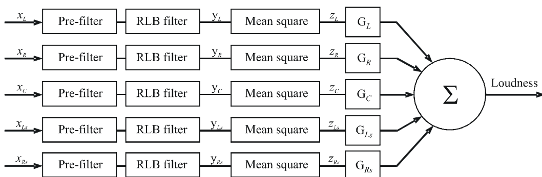
Block diagram of multichannel loudness algorithm
